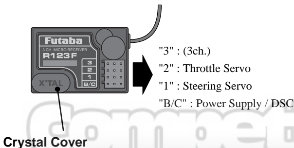
Receiver R123F
