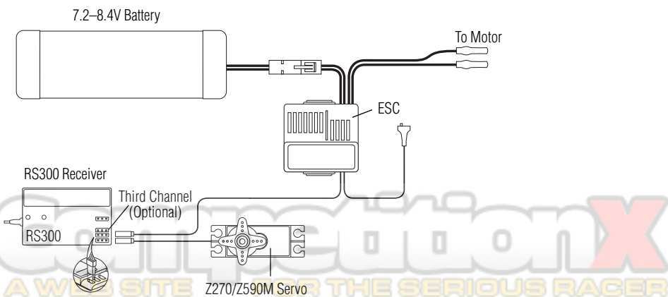
Figure B – Connections to BEC receiver with electronic speed controller. Ni-Cd battery and speed controller are not included in the radio set.
